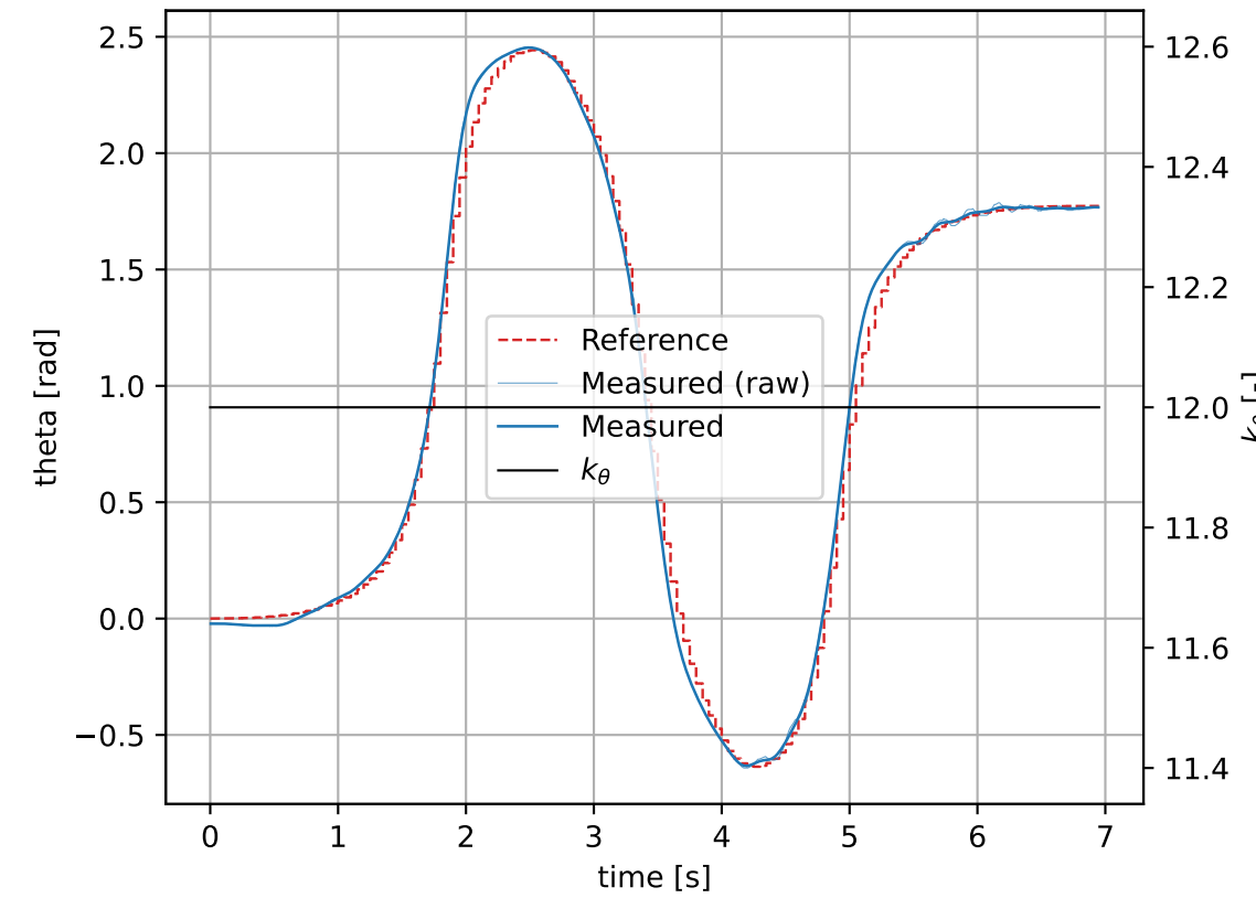
theta State
