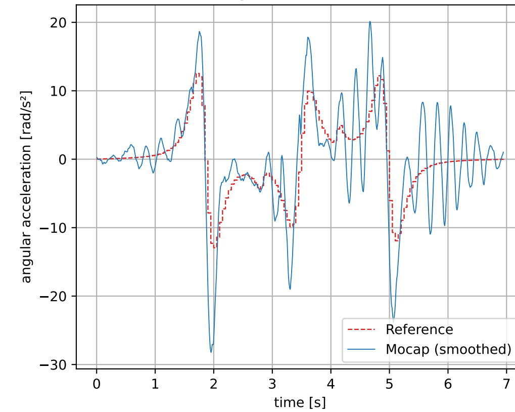
Angular Acceleration
