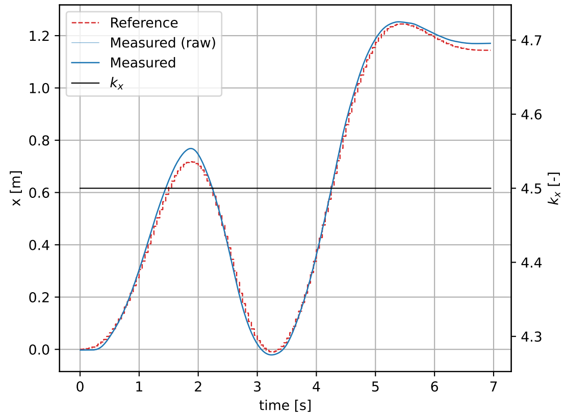
x State
